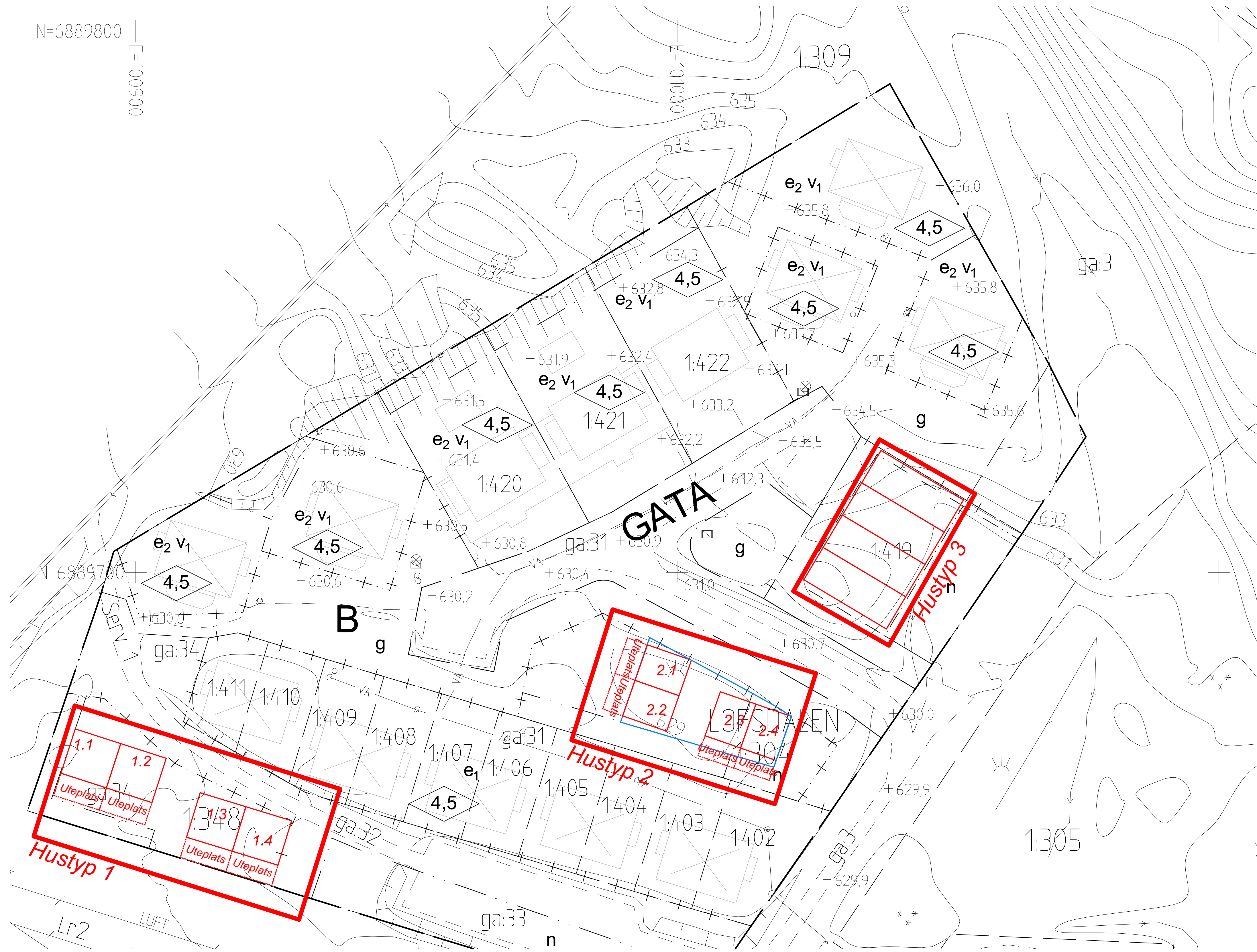
Situationsplan 1:400
